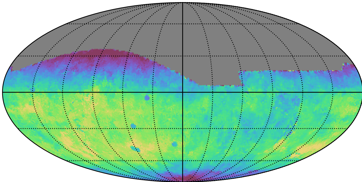
weather_cloudso0v3.4_10yrs All sky g band: Median fiveSigmaDepth
