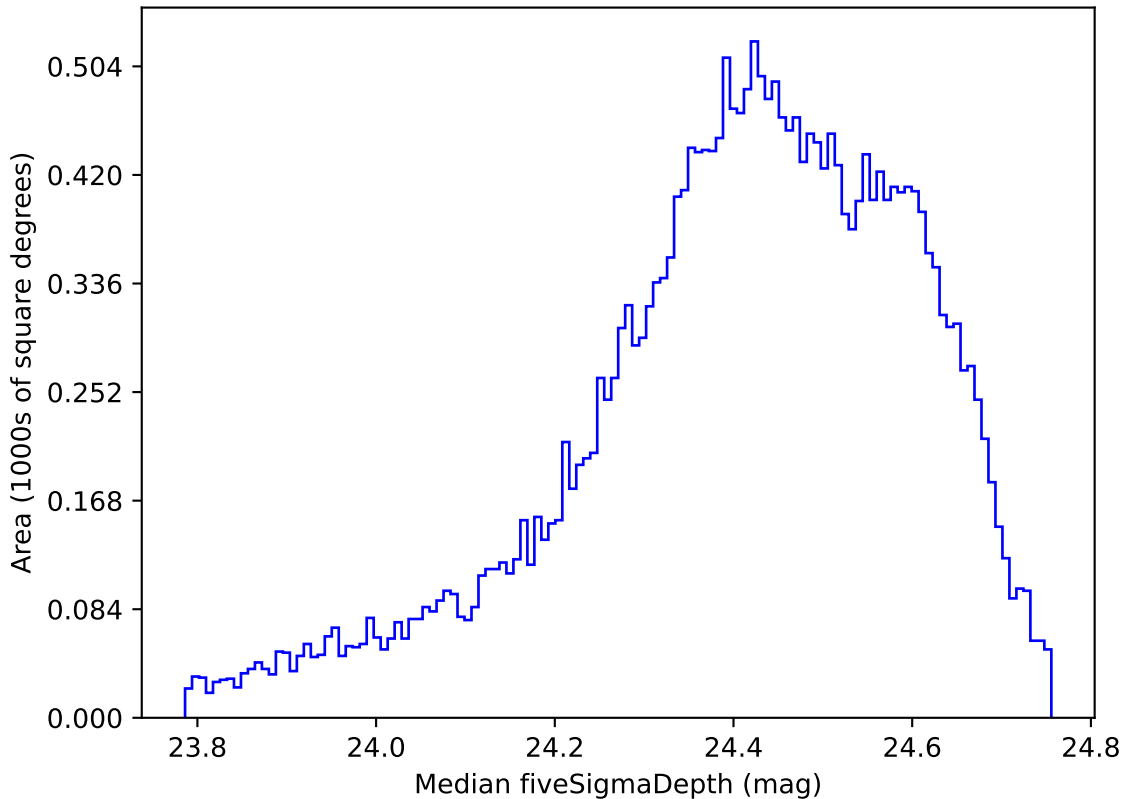
weather_cloudso0v3.4_10yrs All sky g band: Median fiveSigmaDepth
