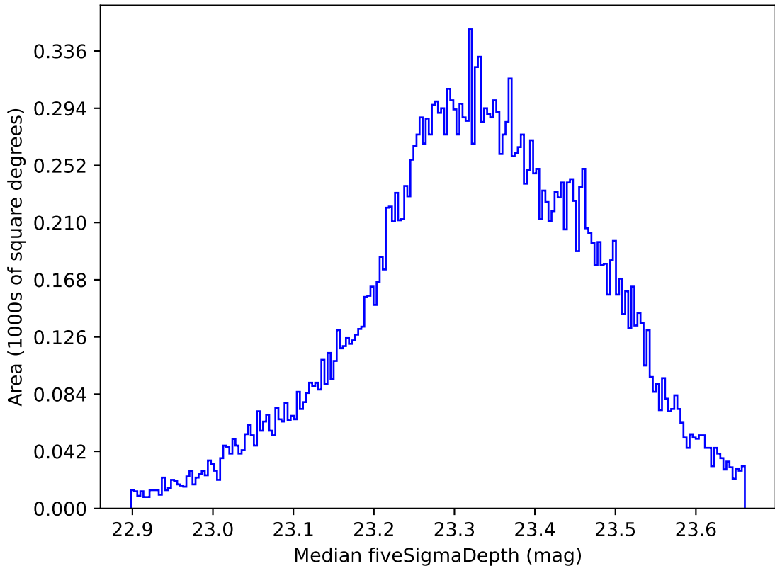
weather_cloudso0v3.4_10yrs All sky all bands: Median fiveSigmaDepth
