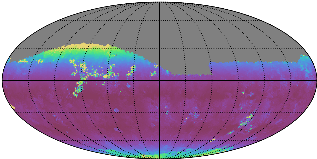
weather_cloudso0v3.4_10yrs Yr 1 z band: Median airmass
