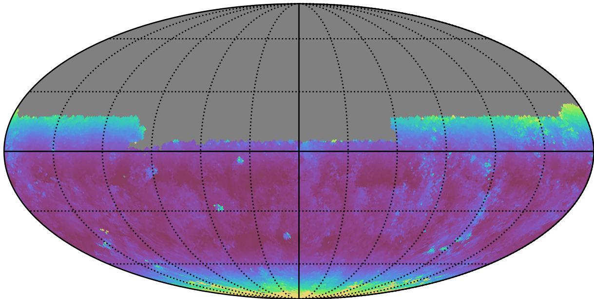
weather_cloudso0v3.4_10yrs Yr 1 y band: Median airmass
