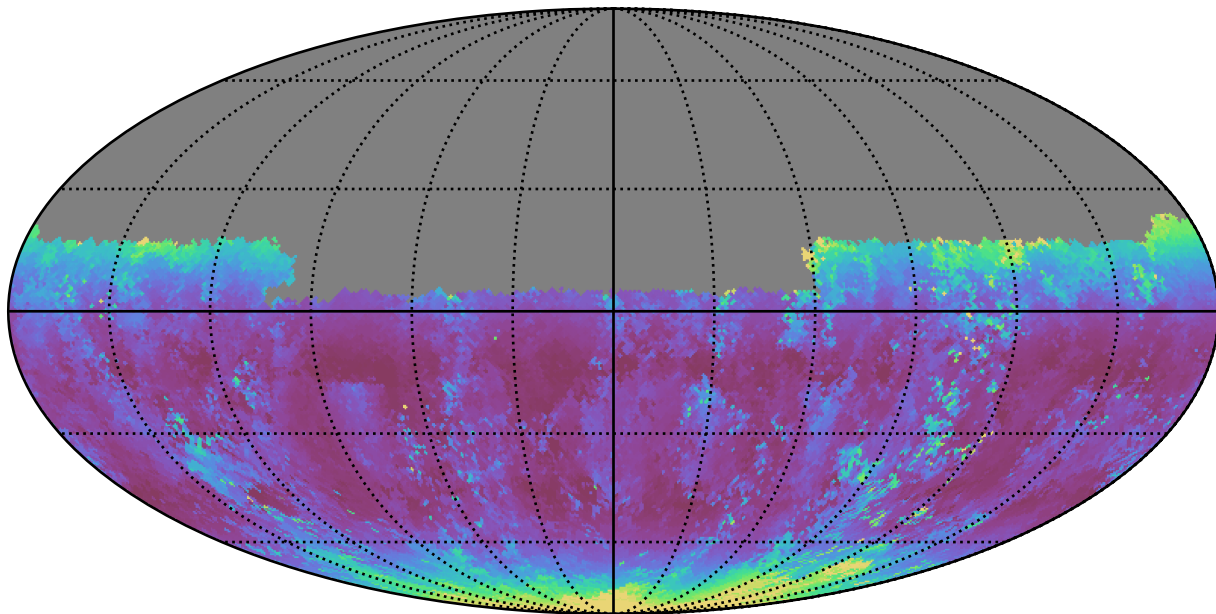
weather_cloudso0v3.4_10yrs Yr 1 u band: Median airmass
