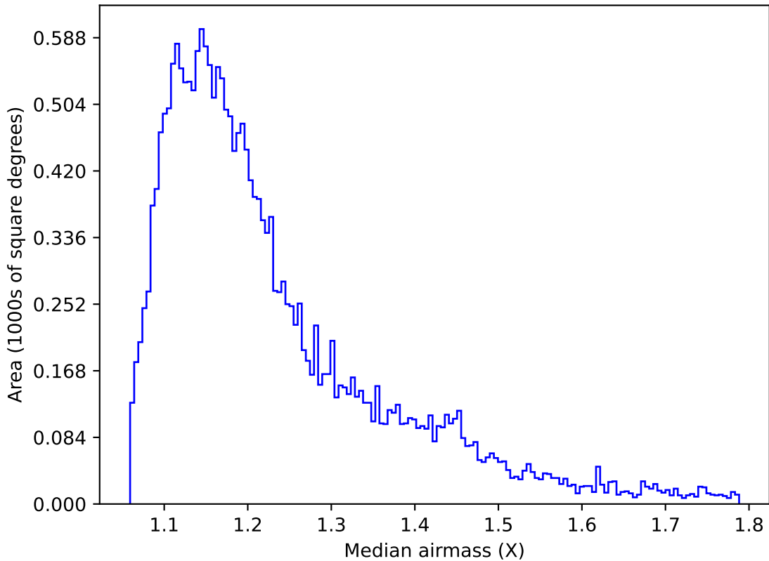
weather_cloudso0v3.4_10yrs Yr 1 u band: Median airmass
