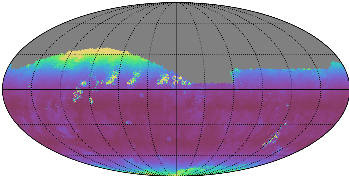
weather_cloudso0v3.4_10yrs Yr 1 r band: Median airmass
