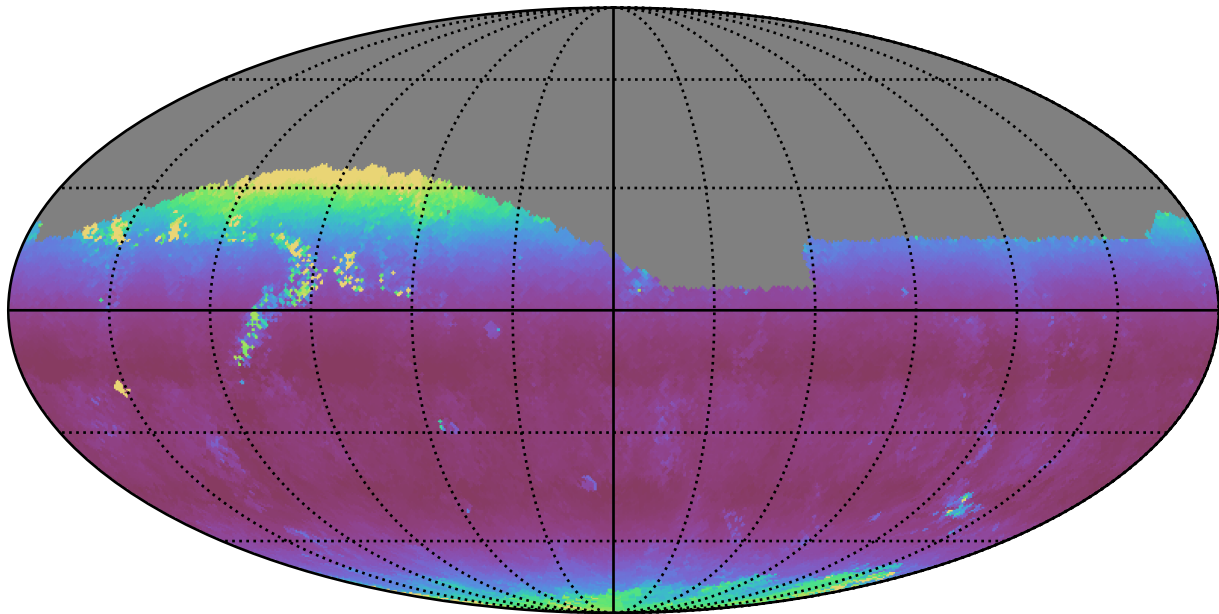
weather_cloudso0v3.4_10yrs Yr 1 i band: Median airmass
