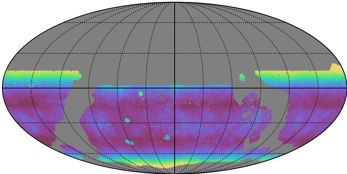
weather_cloudso0v3.4_10yrs WFD z band: Median airmass
