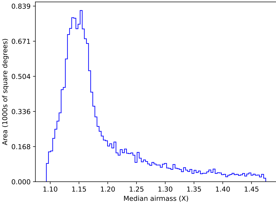
weather_cloudso0v3.4_10yrs WFD y band: Median airmass
