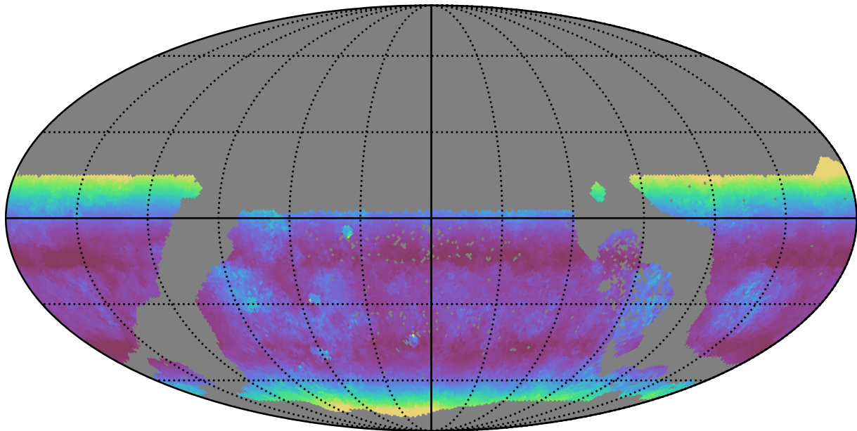
weather_cloudso0v3.4_10yrs WFD u band: Median airmass
