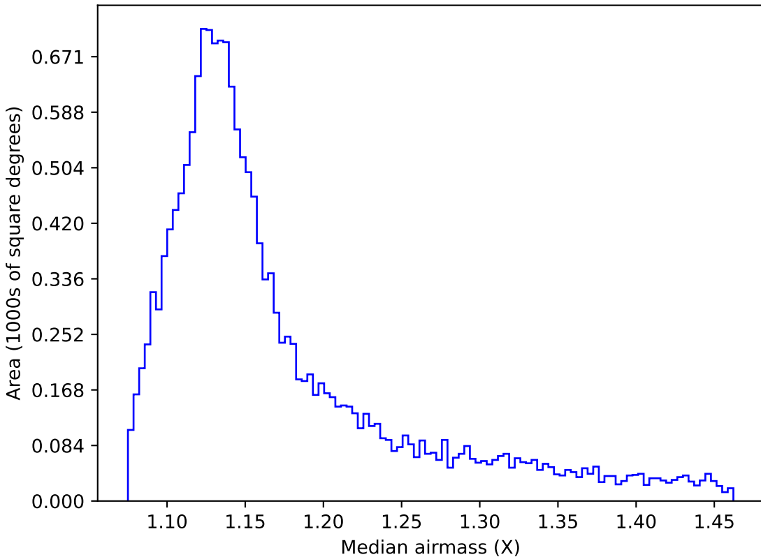
weather_cloudso0v3.4_10yrs WFD r band: Median airmass
