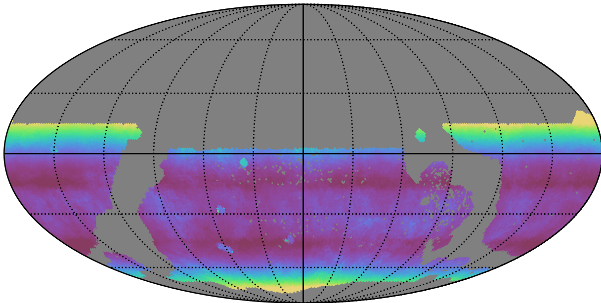
weather_cloudso0v3.4_10yrs WFD i band: Median airmass
