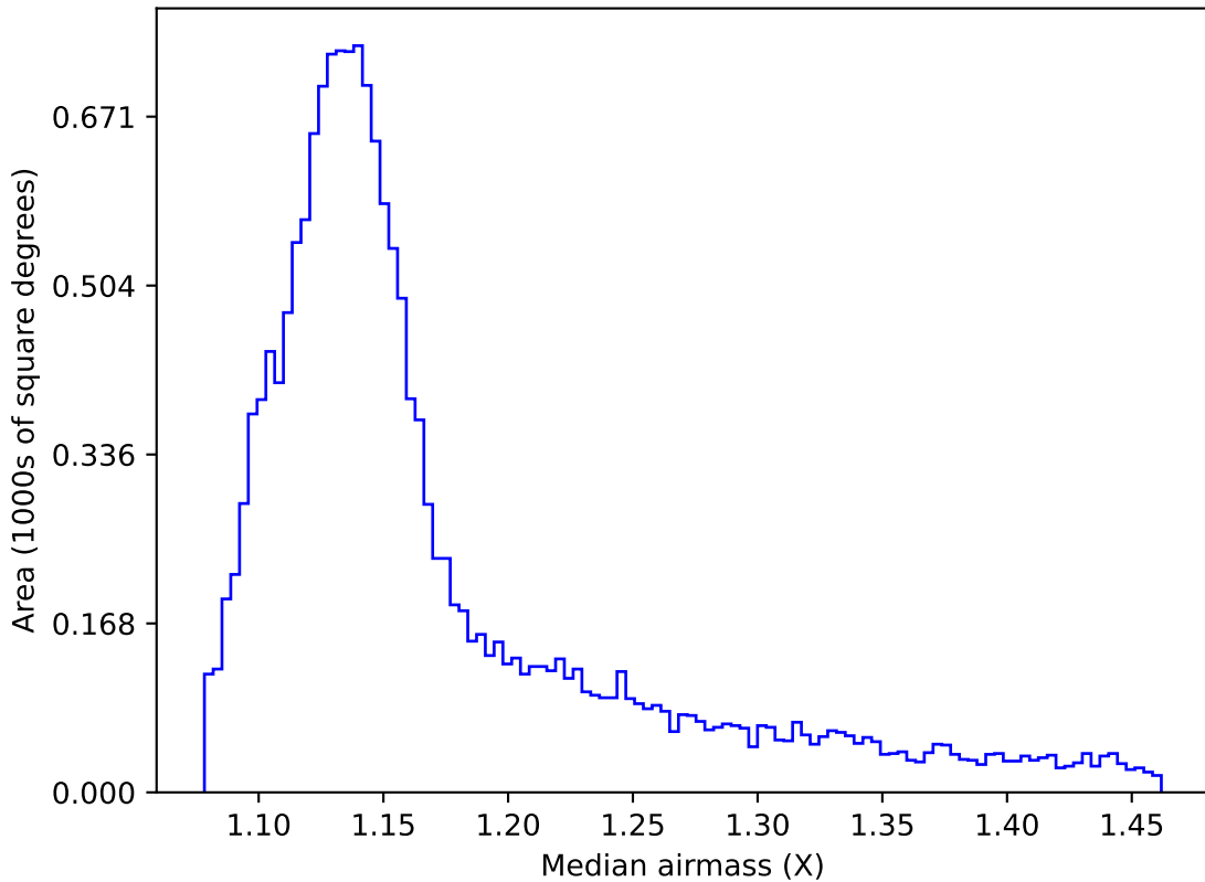
weather_cloudso0v3.4_10yrs WFD i band: Median airmass
