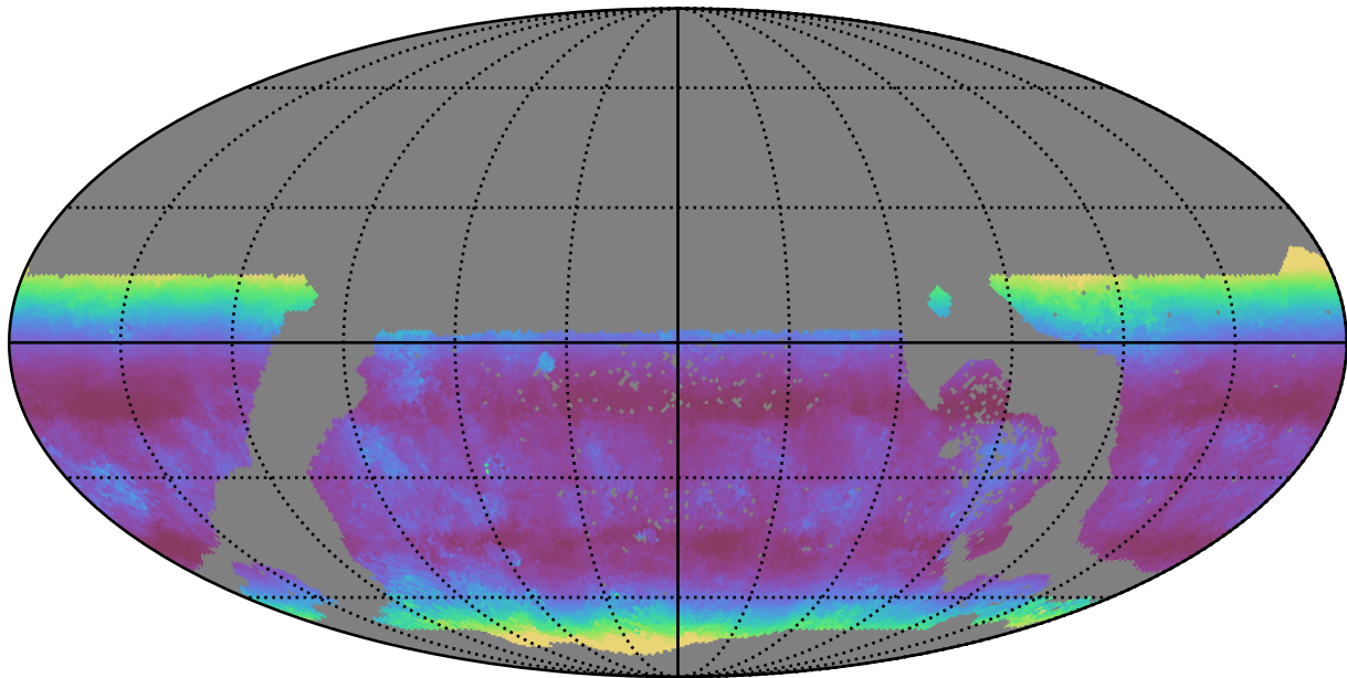
weather_cloudso0v3.4_10yrs WFD g band: Median airmass
