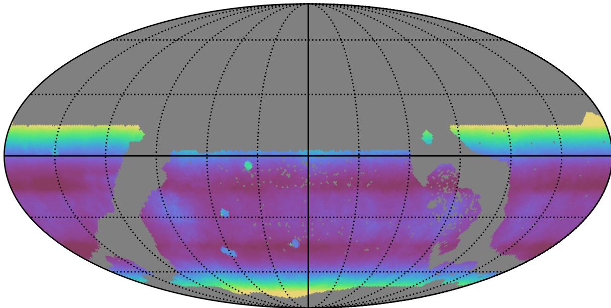
weather_cloudso0v3.4_10yrs WFD all bands: Median airmass
