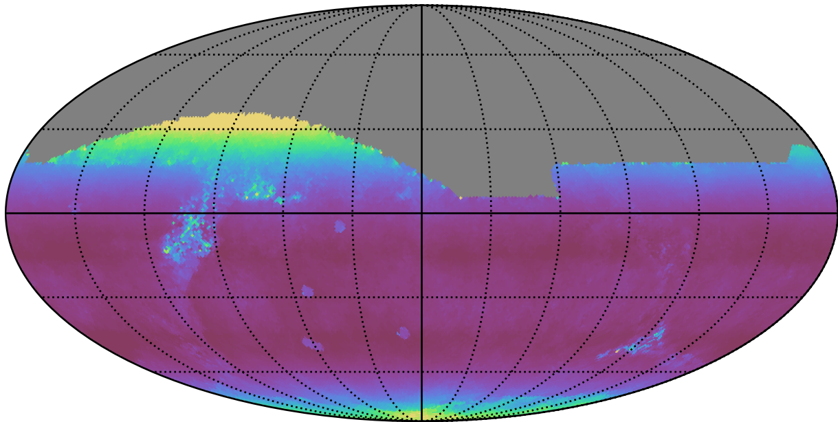
weather_cloudso0v3.4_10yrs All sky z band: Median airmass
