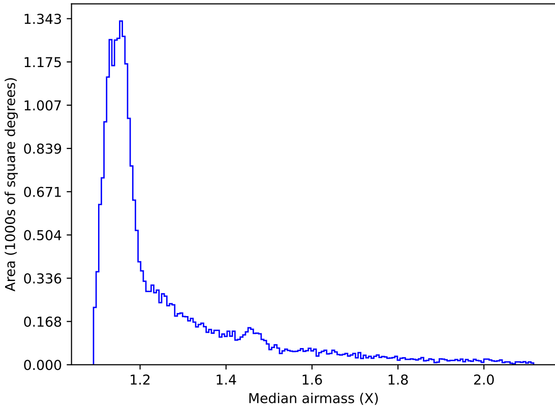
weather_cloudso0v3.4_10yrs All sky z band: Median airmass
