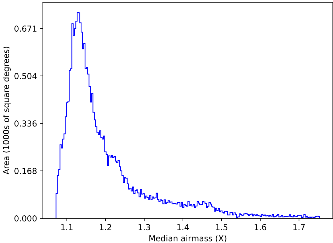
weather_cloudso0v3.4_10yrs All sky u band: Median airmass
