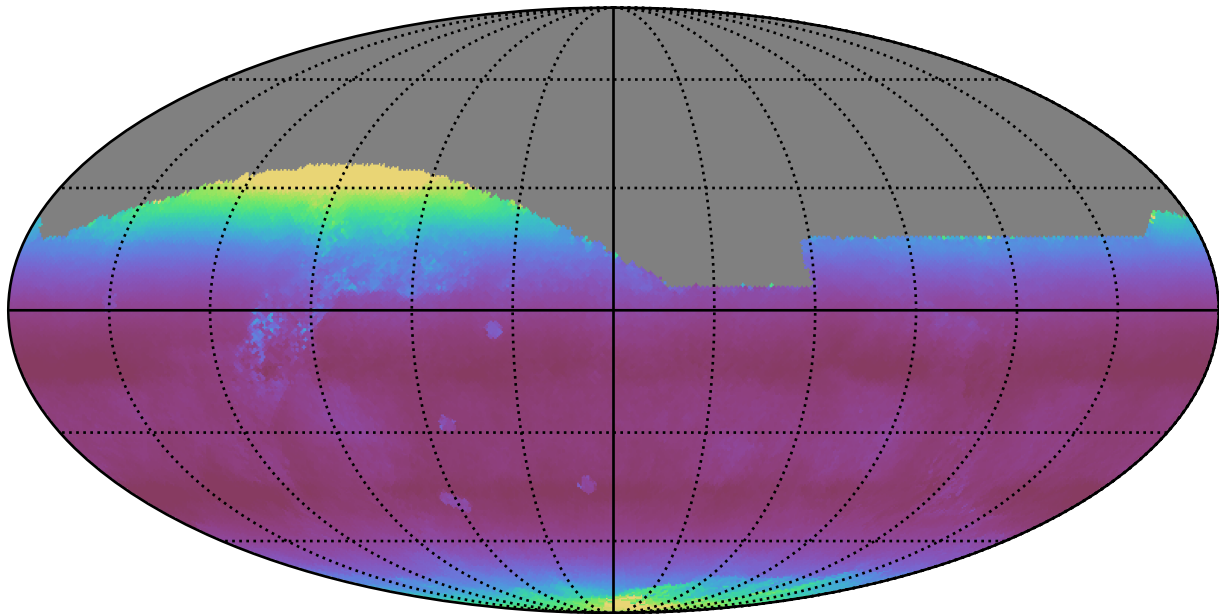
weather_cloudso0v3.4_10yrs All sky r band: Median airmass
