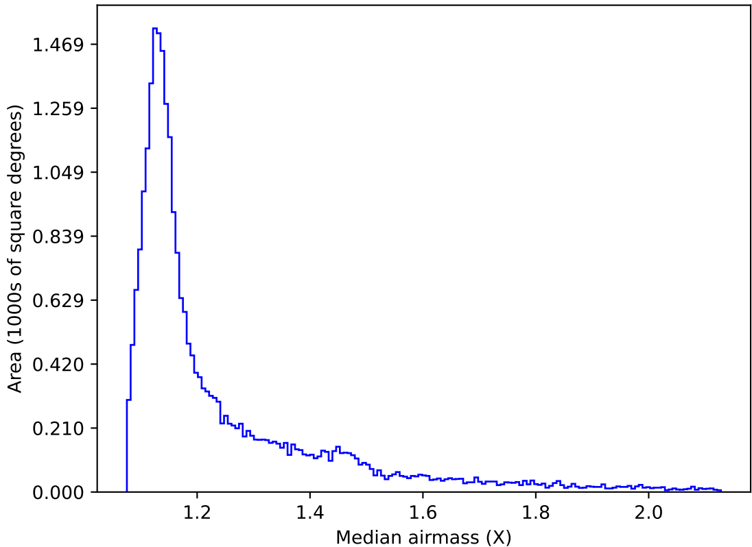
weather_cloudso0v3.4_10yrs All sky r band: Median airmass
