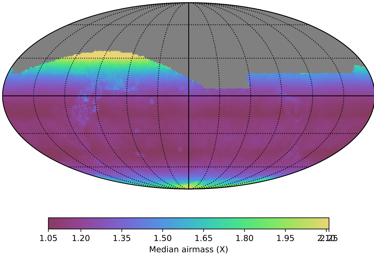
weather_cloudso0v3.4_10yrs All sky i band: Median airmass
