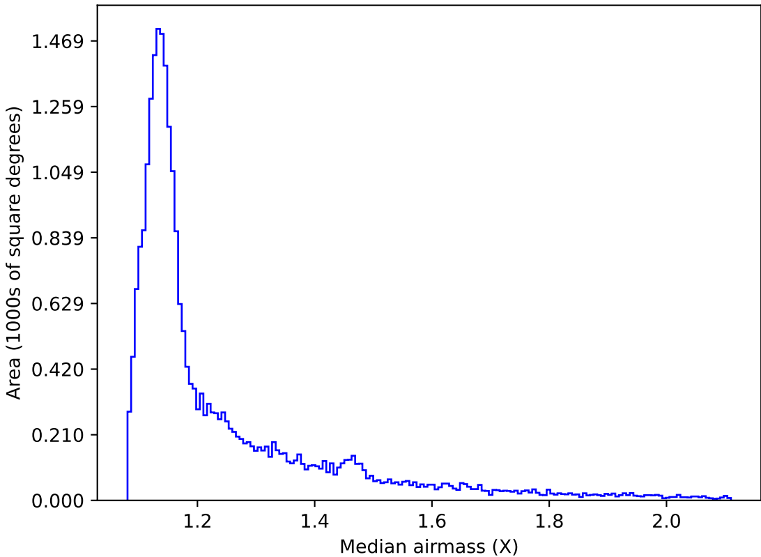
weather_cloudso0v3.4_10yrs All sky i band: Median airmass
