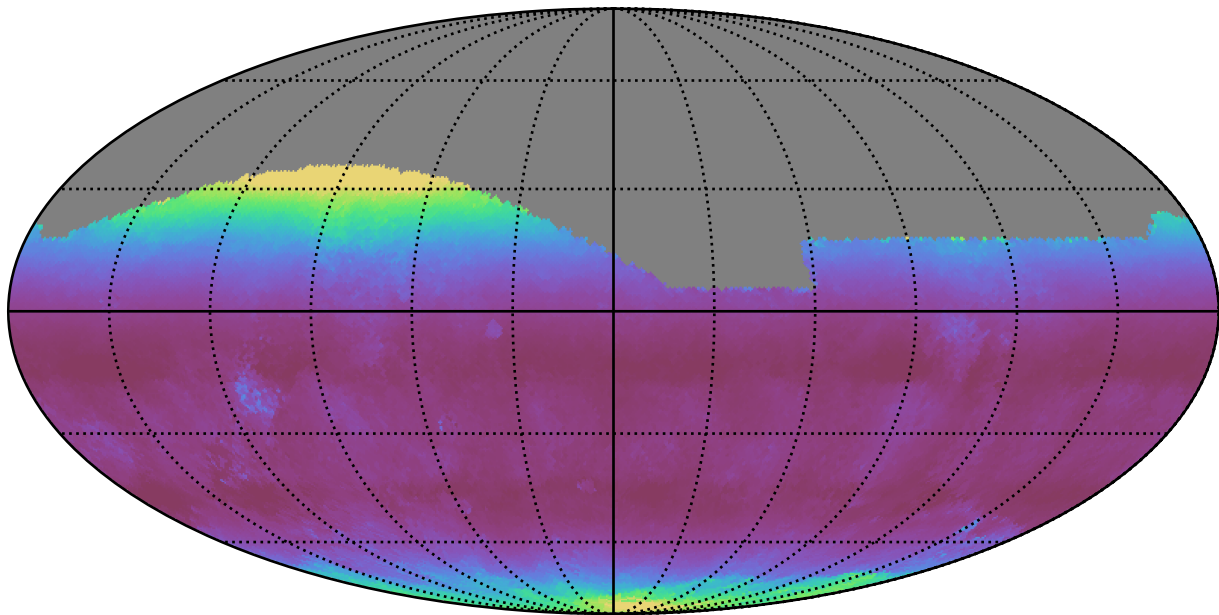
weather_cloudso0v3.4_10yrs All sky g band: Median airmass
