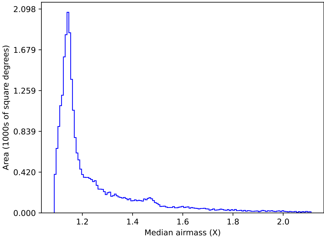
weather_cloudso0v3.4_10yrs All sky all bands: Median airmass
