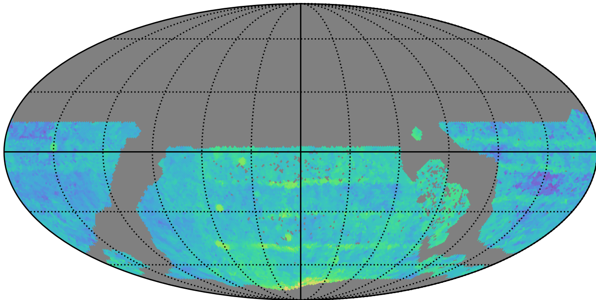
weather_cloudso0v3.4_10yrs WFD z band: Median Season Length
