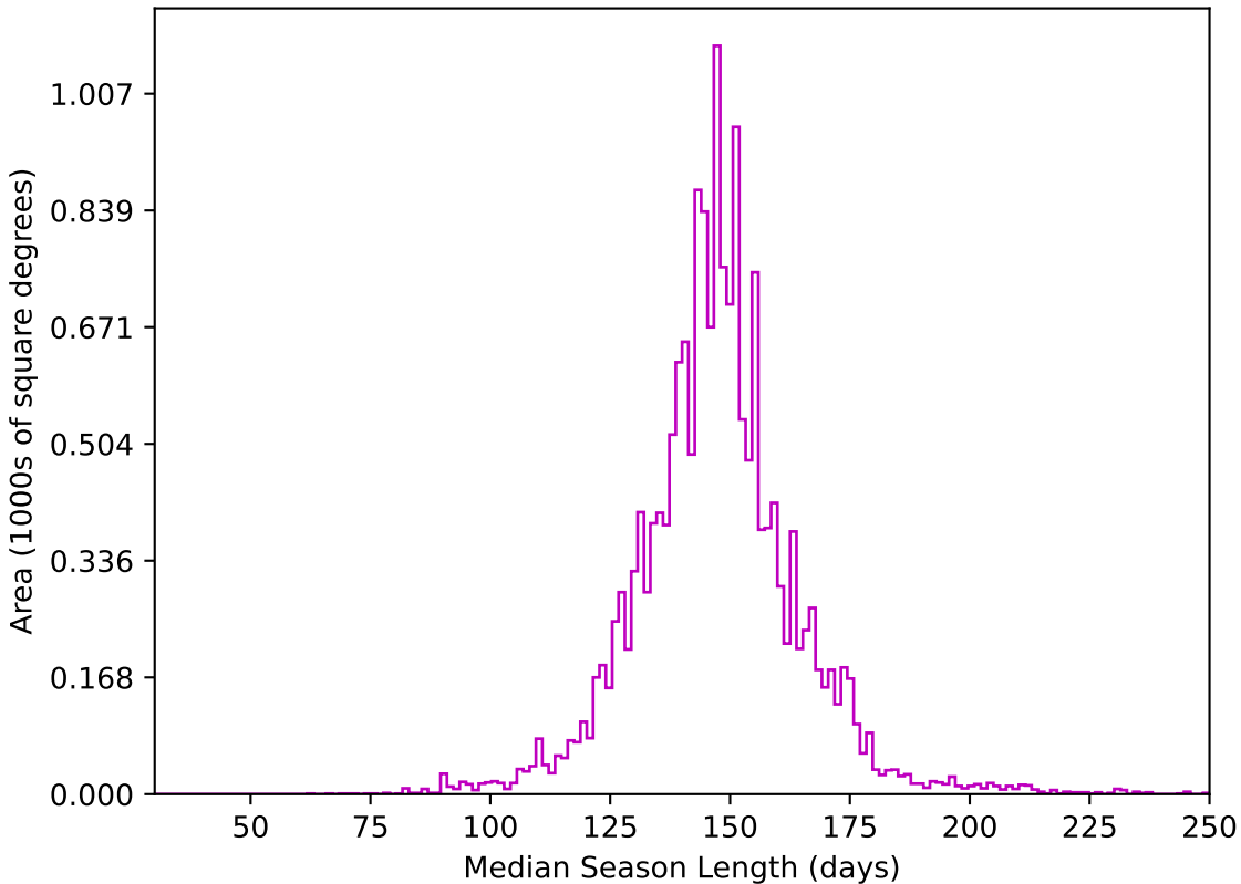
weather_cloudso0v3.4_10yrs WFD z band: Median Season Length
