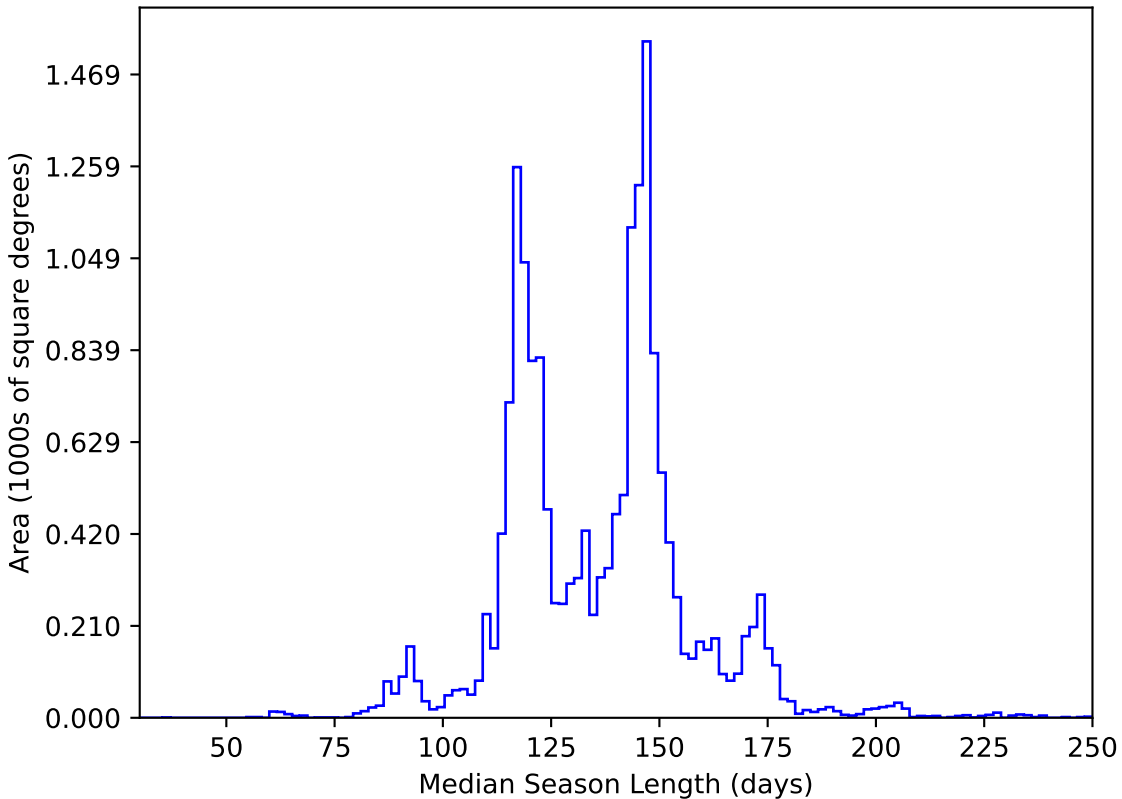
weather_cloudso0v3.4_10yrs WFD y band: Median Season Length
