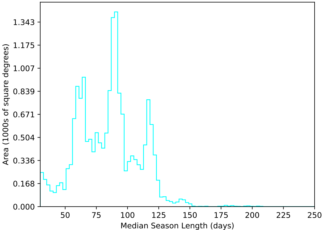
weather_cloudso0v3.4_10yrs WFD u band: Median Season Length
