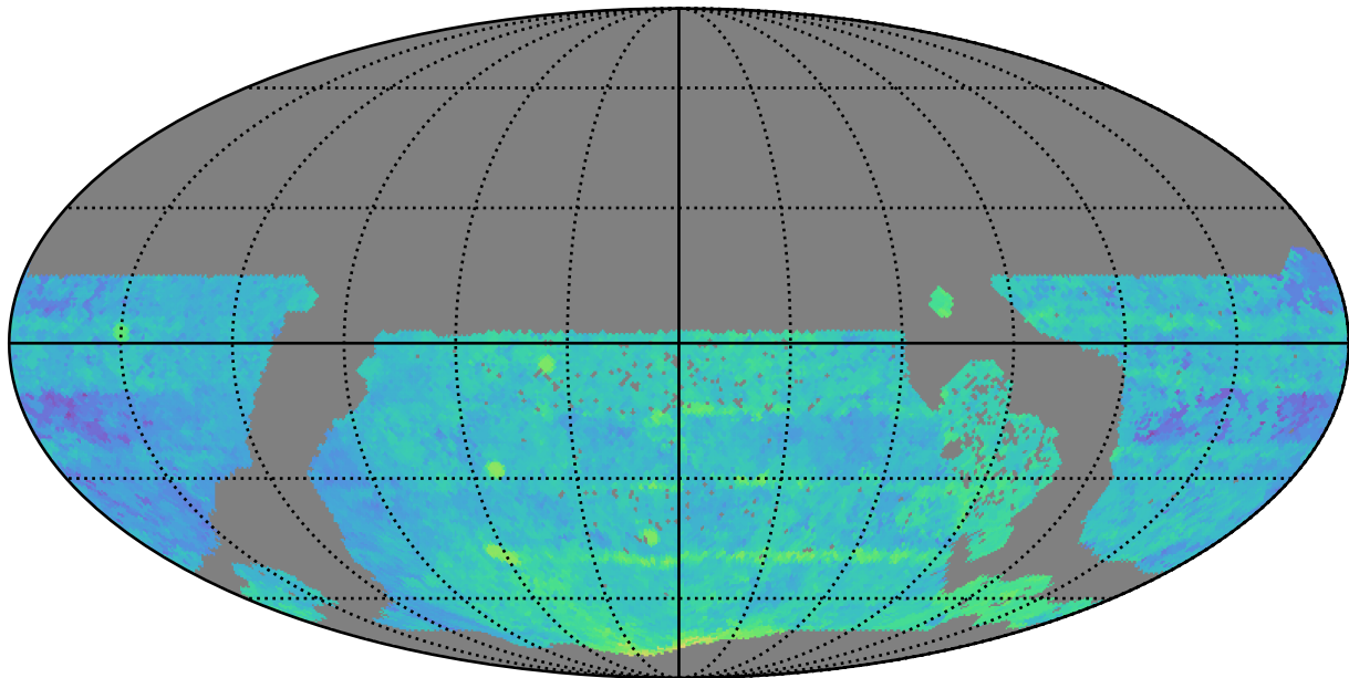
weather_cloudso0v3.4_10yrs WFD i band: Median Season Length
