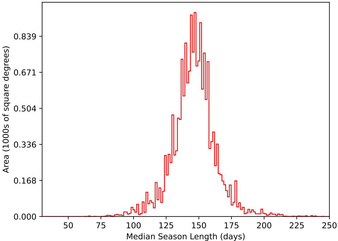
weather_cloudso0v3.4_10yrs WFD i band: Median Season Length
