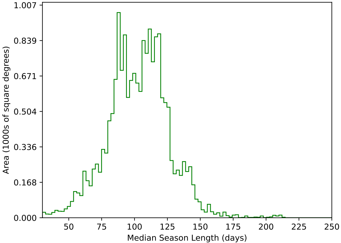
weather_cloudso0v3.4_10yrs WFD g band: Median Season Length
