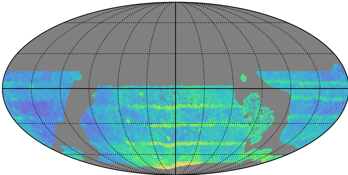
weather_cloudso0v3.4_10yrs WFD all bands: Median Season Length
