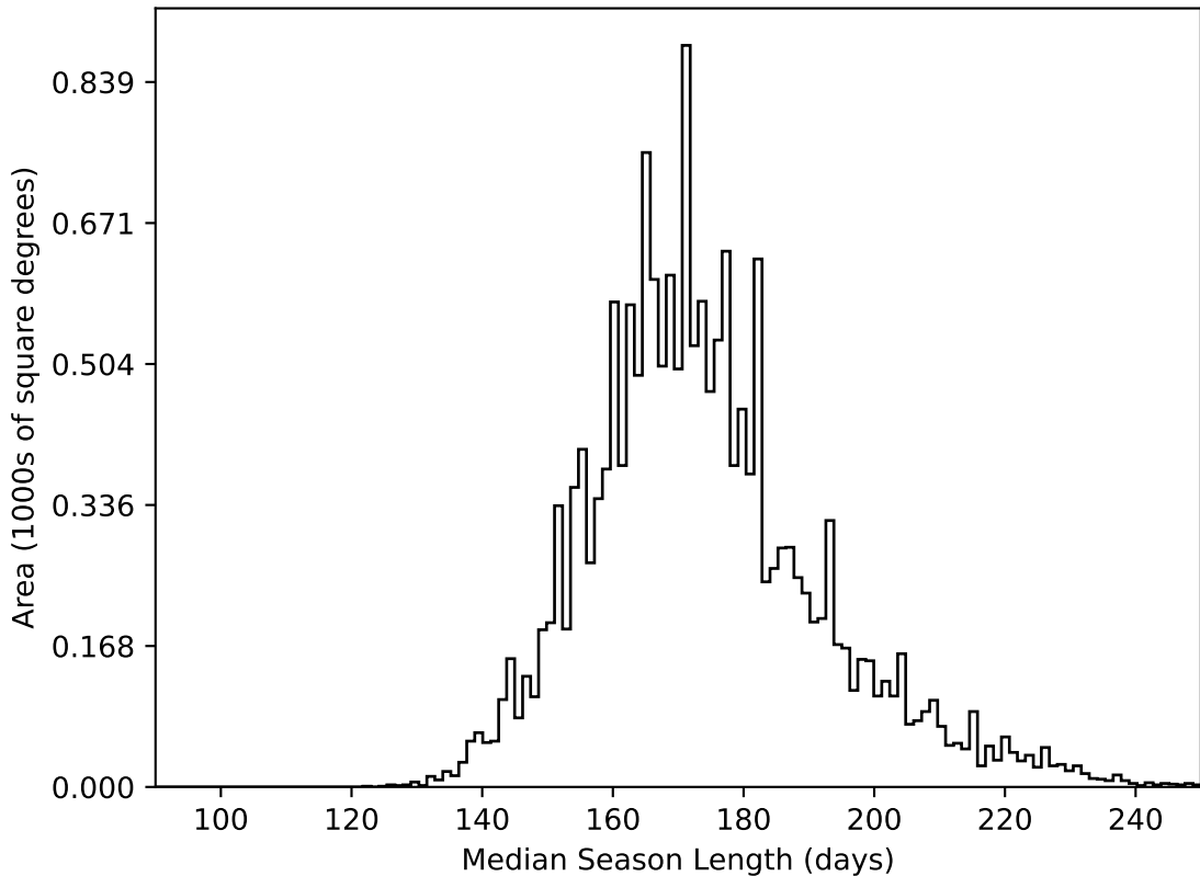
weather_cloudso0v3.4_10yrs WFD all bands: Median Season Length
