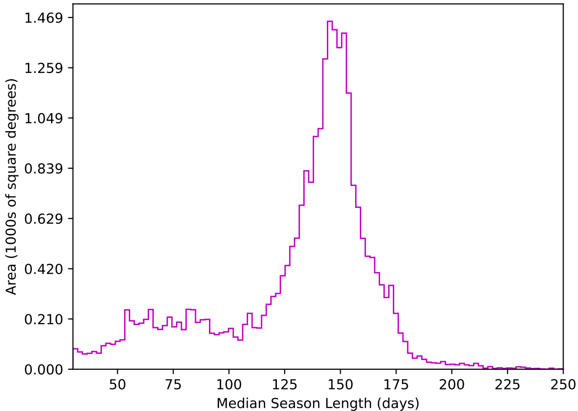
weather_cloudso0v3.4_10yrs All sky z band: Median Season Length
