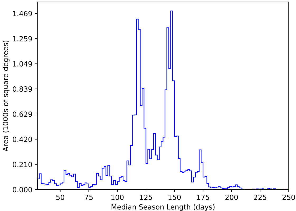
weather_cloudso0v3.4_10yrs All sky y band: Median Season Length
