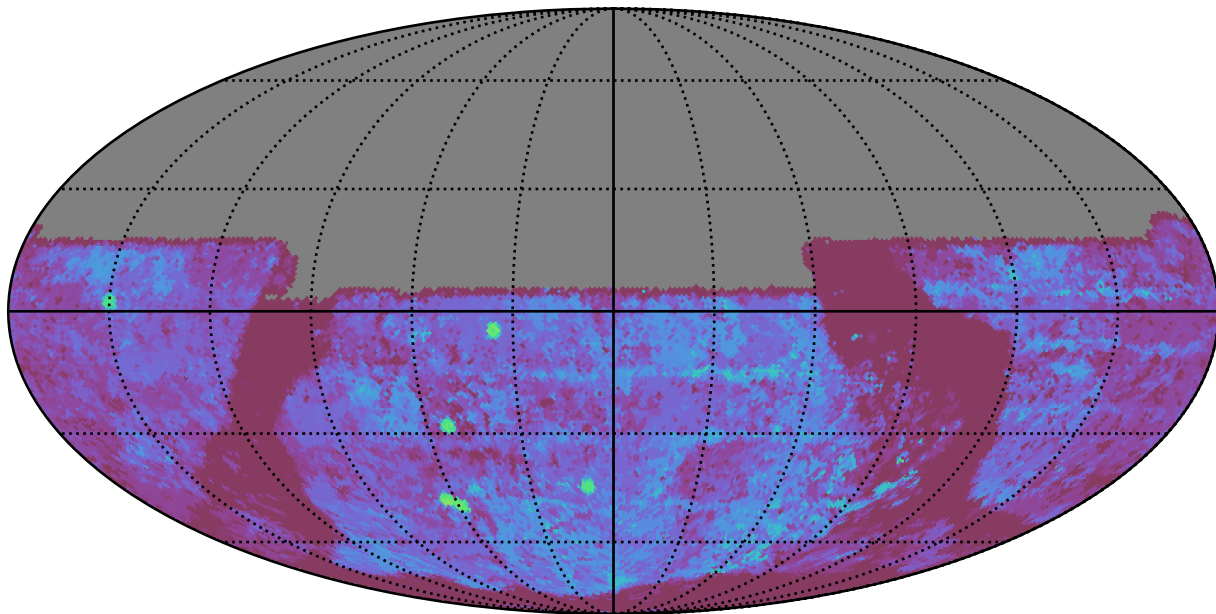
weather_cloudso0v3.4_10yrs All sky u band: Median Season Length
