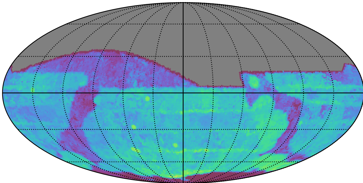
weather_cloudso0v3.4_10yrs All sky r band: Median Season Length
