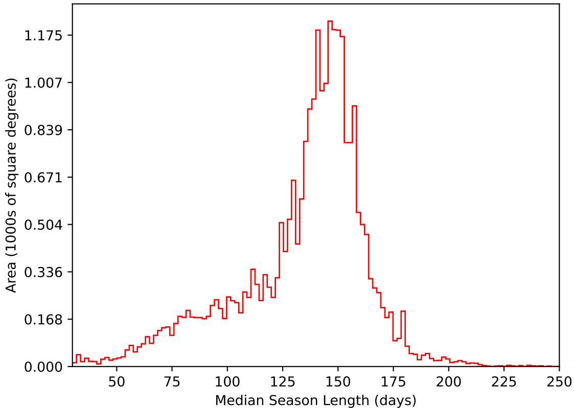
weather_cloudso0v3.4_10yrs All sky i band: Median Season Length
