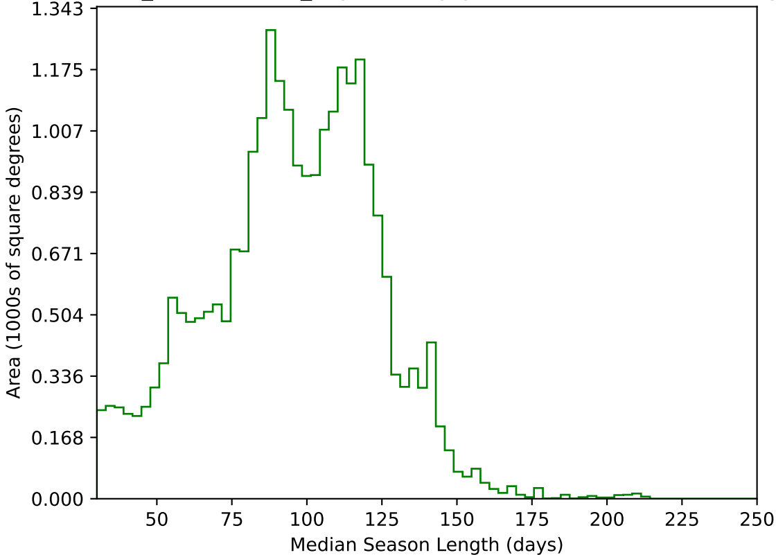
weather_cloudso0v3.4_10yrs All sky g band: Median Season Length
