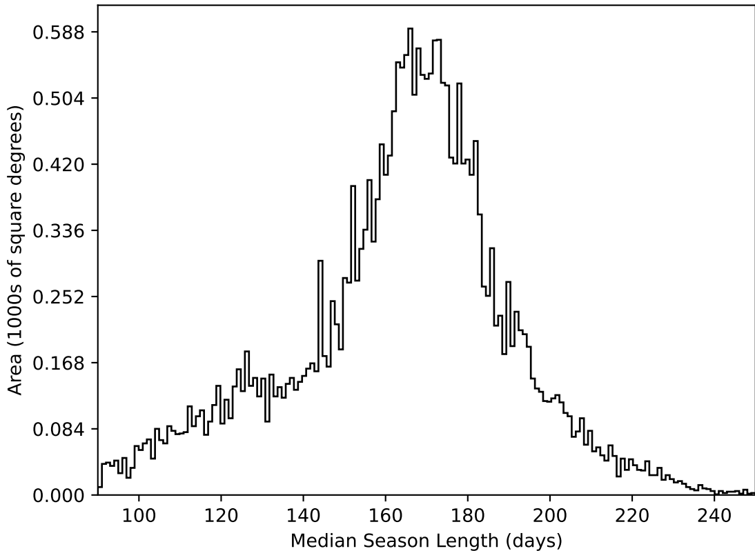
weather_cloudso0v3.4_10yrs All sky all bands: Median Season Length
