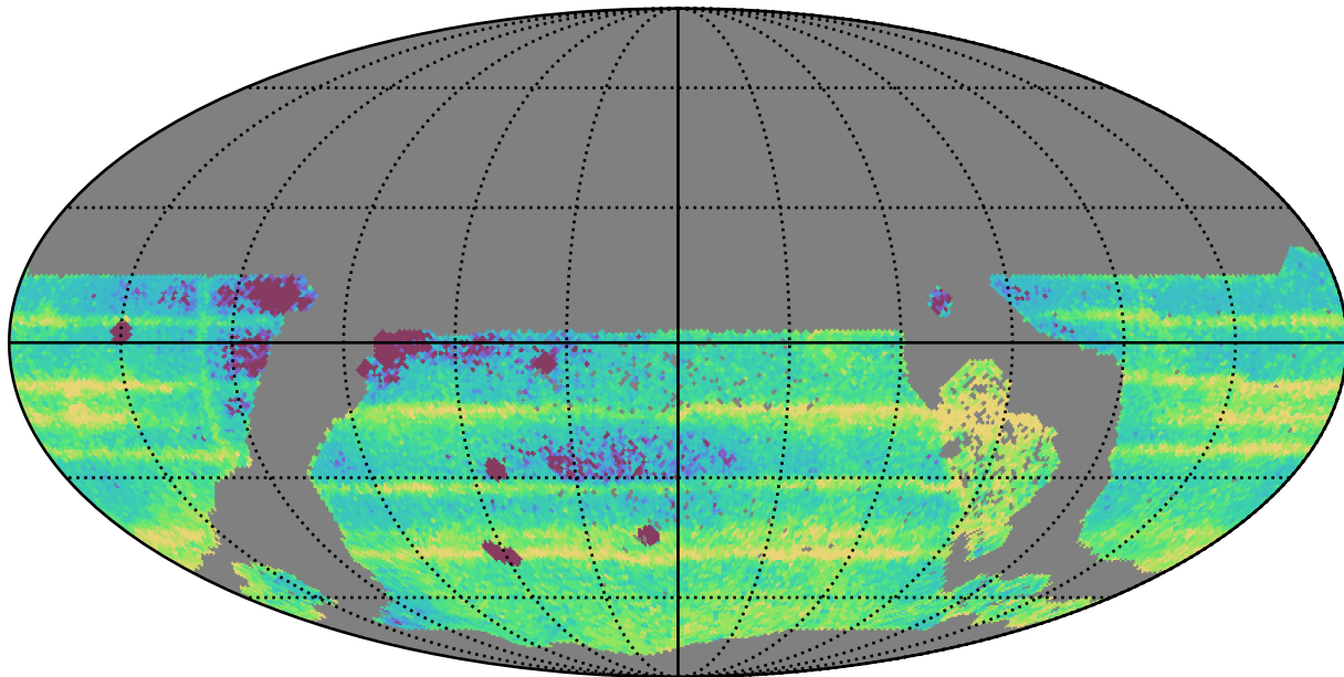
weather_cloudso0v3.4_10yrs WFD: Median Intra-Night Gap
