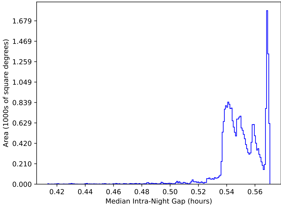
weather_cloudso0v3.4_10yrs All sky: Median Intra-Night Gap
