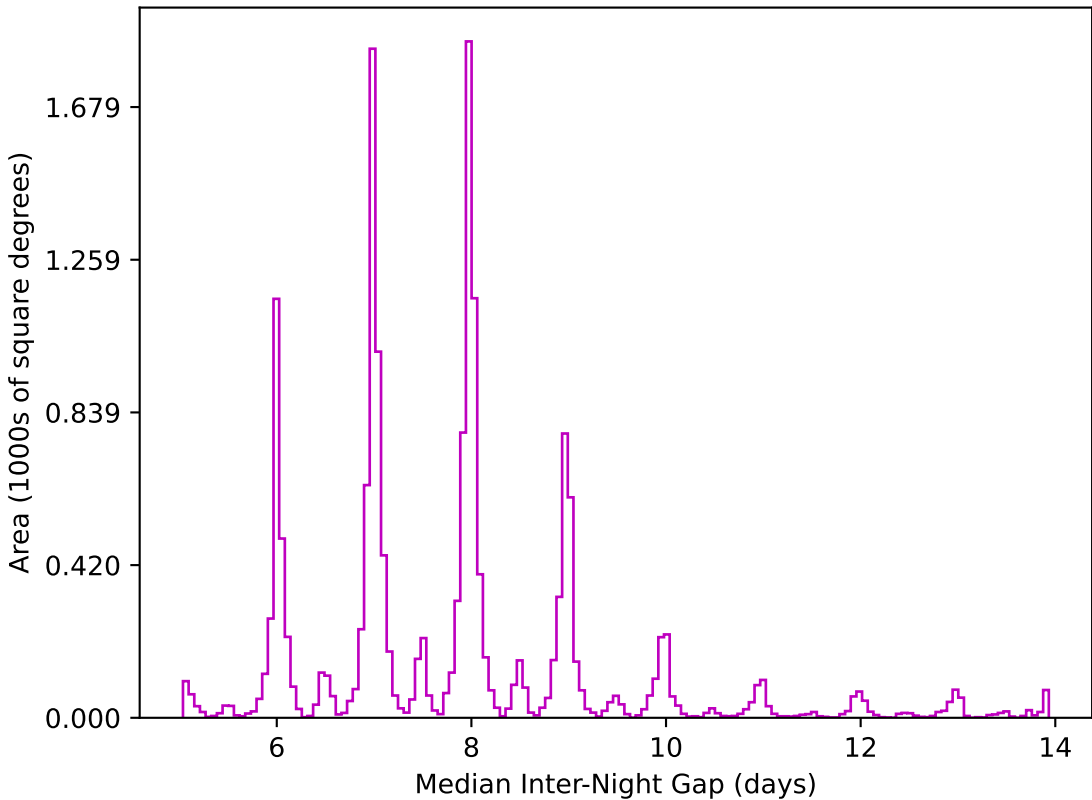
weather_cloudso0v3.4_10yrs WFD z band: Median Inter-Night Gap
