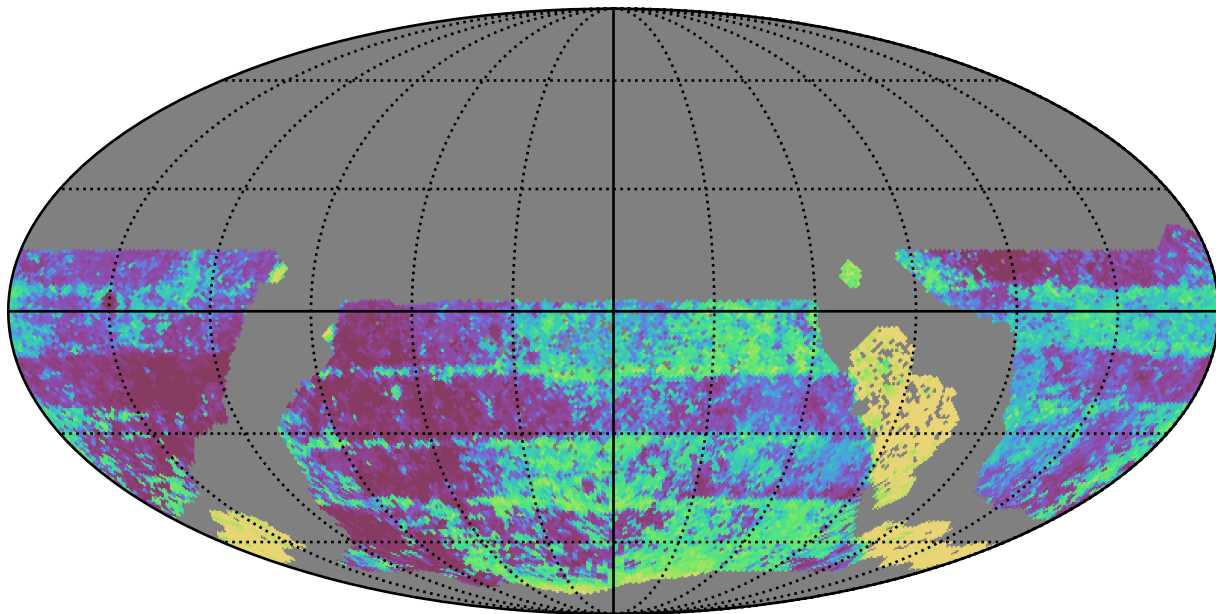
weather_cloudso0v3.4_10yrs WFD y band: Median Inter-Night Gap
