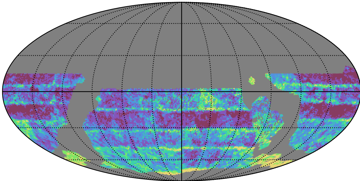
weather_cloudso0v3.4_10yrs WFD r band: Median Inter-Night Gap
