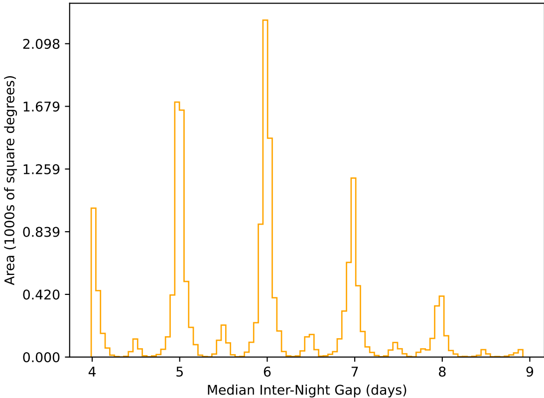
weather_cloudso0v3.4_10yrs WFD r band: Median Inter-Night Gap
