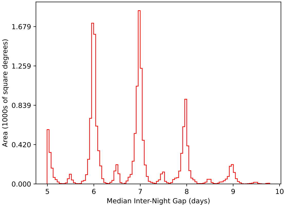
weather_cloudso0v3.4_10yrs WFD i band: Median Inter-Night Gap
