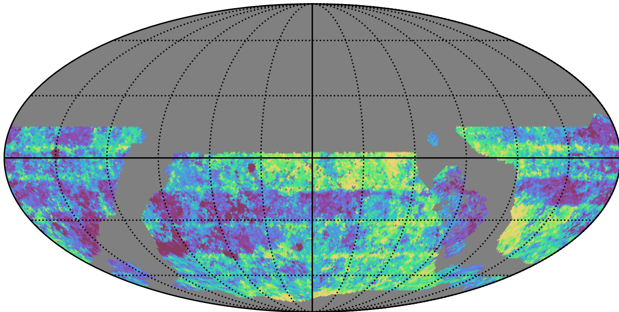
weather_cloudso0v3.4_10yrs WFD g band: Median Inter-Night Gap
